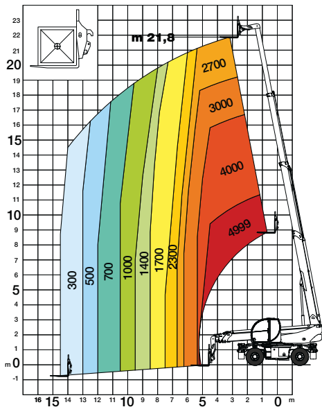
Frontal position load chart on tyres with forks
